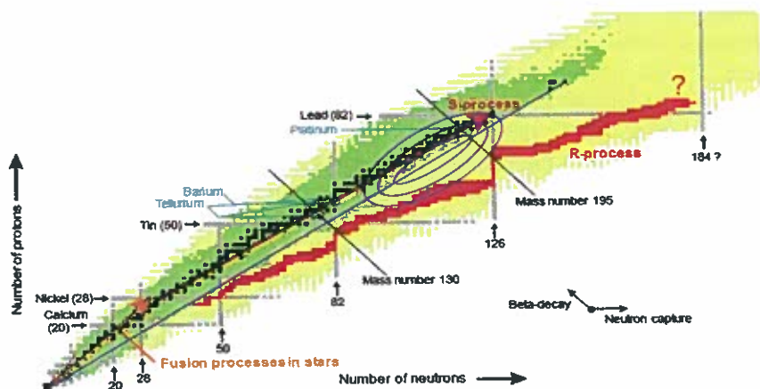
Figure 3. Nuclidic chart, showing the different nucleosynthesis processes like the r -process, the s -process, or the fusion processes in stars together with contour lines of the new fission-fusion process for producing very neutron-rich nuclei close to N = 126 waiting point of the r -process.
