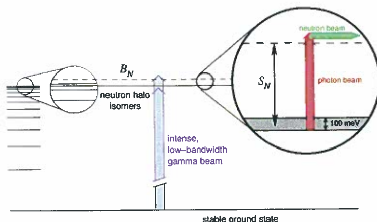
Figure 5. Schematic picture of the new neutron production scheme, using the \gamma -beam to excite neutron-halo isomers with a neutron separation energy S_N below the binding energy E_B . The left level scheme shows the increasing number of compound nuclear resonances as a function of the excitation energy. The halo isomer is fragmented into several high-lying resonances, resulting in halo isomers with different binding energies. The two blue arrows indicate the width of the \gamma beam. Then in a second step, a photon beam of much lower energy, shown in red, generates the neutron beam by dissociating the neutron halo states.
