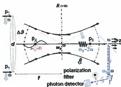
Figure 4. Suggested experimental setup to detect low-mass elementary particles by mediating the two-photon transition in vacuum of an intense laser focus.
