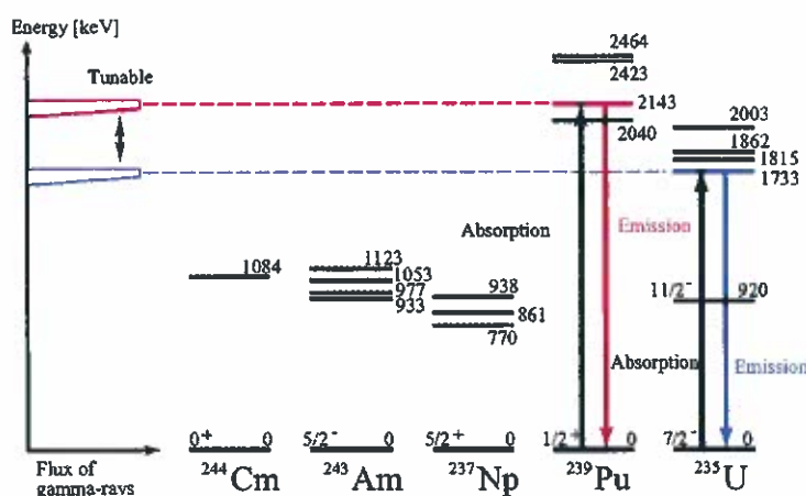
Figure 6. Nuclear resonance fluorescence of several actinides, demonstrating the high sensitivity of the method [26].
